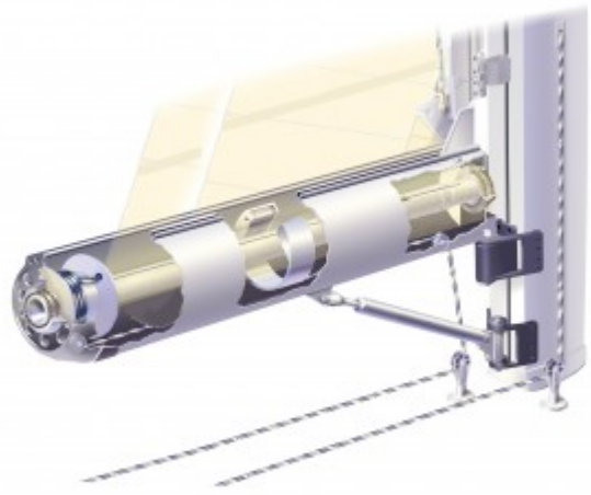
BoomFurl w/ sail Drawing JPEG
